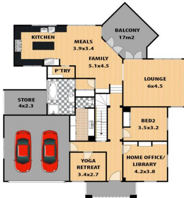
ENTRY LEVEL
